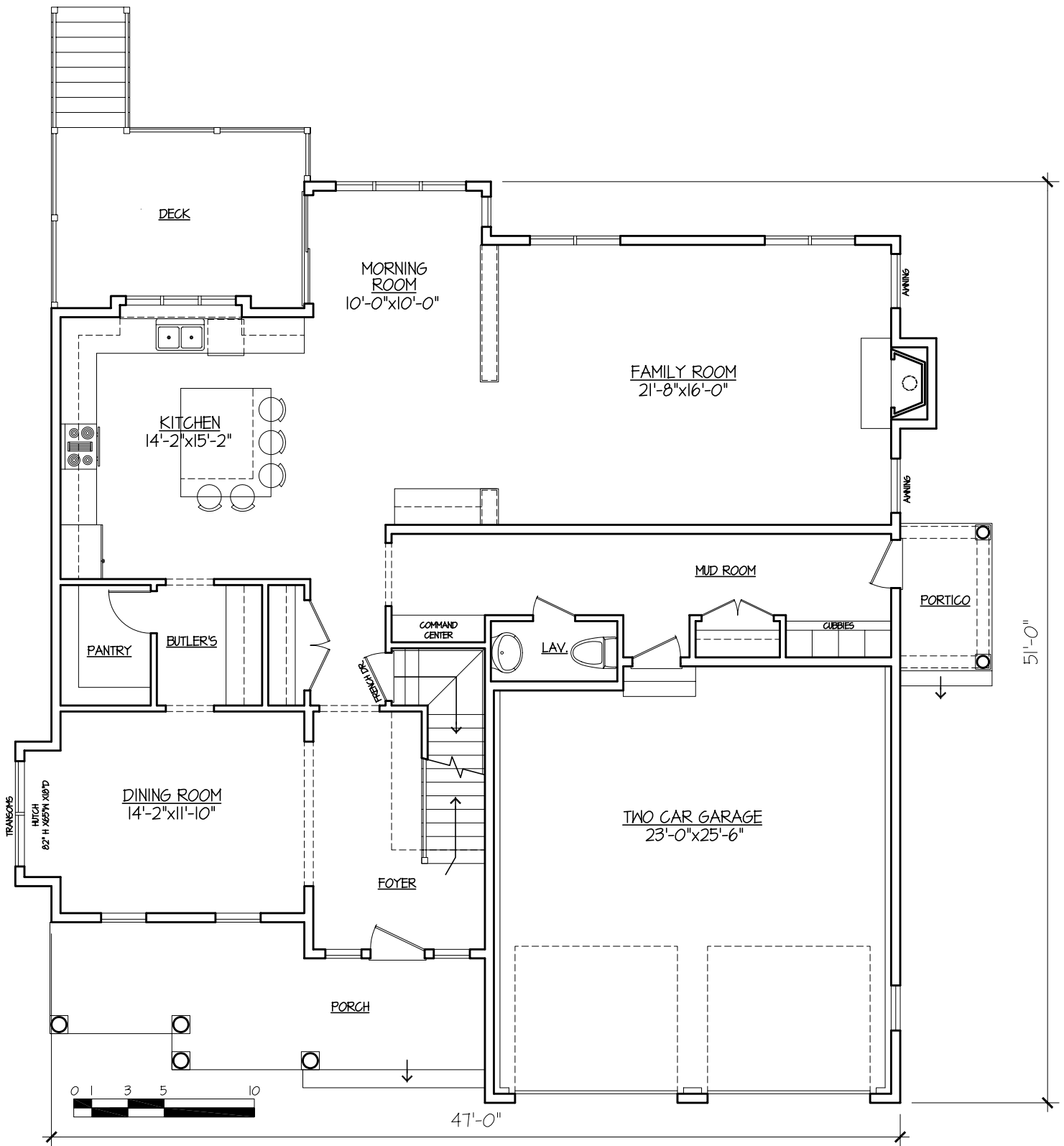
PROPOSED FIRST FLOOR PLAN 1473 SQFT 7-30-10
